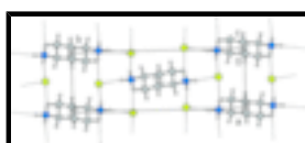
Fig. 3. Crystal packing seen along the c direction. Hydrogen bonding interactions are shown as dotted lines.
