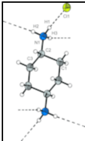
Fig. 1. The structure of the title compound (displacement ellipsoids at the 40% probability level, H-atoms drawn with arbitrary radius). Thin dashed lines show hydrogen bonds to neighbouring chloride anions. The atoms of the asymmetric unit are labeled.
